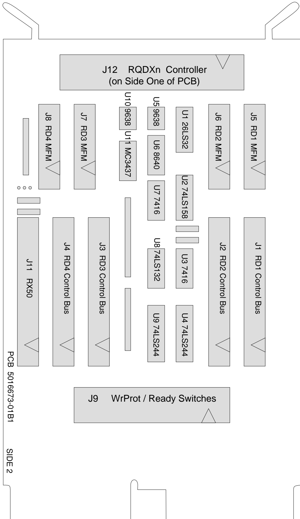
M9058 RQDX Signal Distribution - Approximate layout, as seen from below. Drawn Feb.1993 P.N.T.
