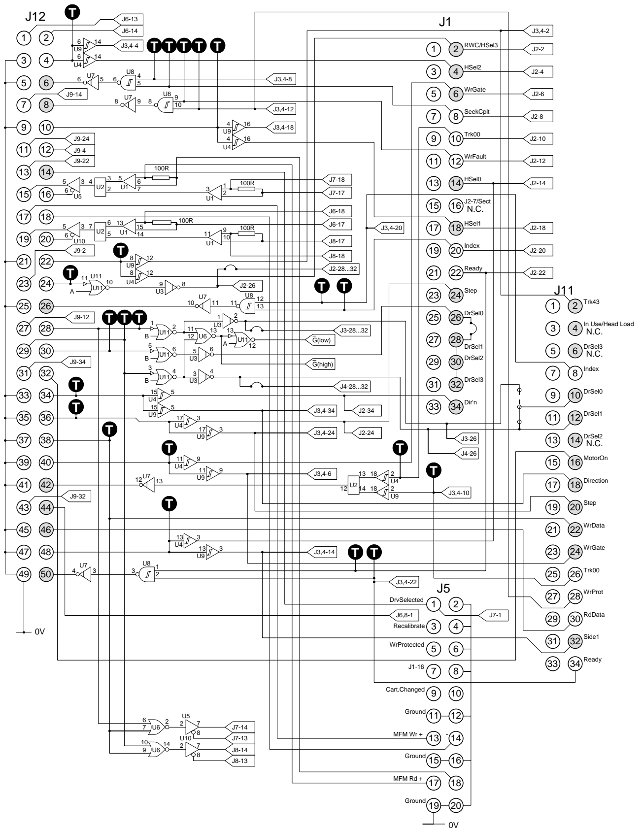
M9058 RQDX Signal Distribution
